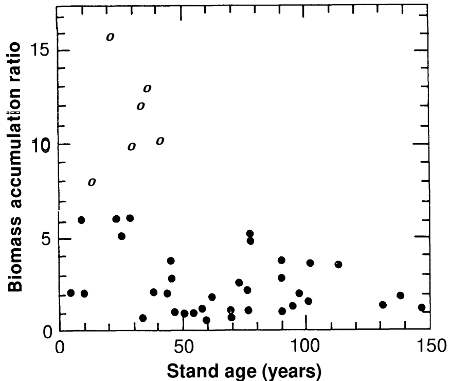
Figure 5.—Changes in understory biomass structure during secondary succession. Biomass accumulation ratio = annual production/total aboveground biomass.
