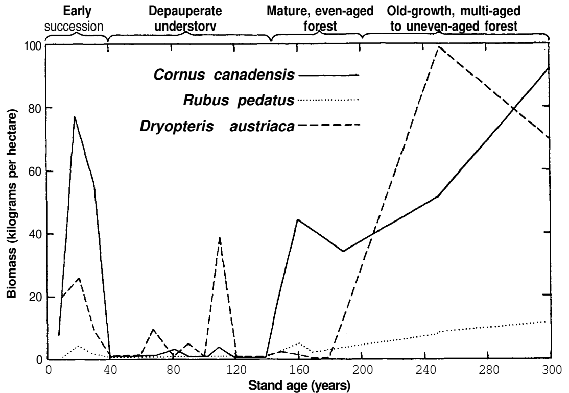
Figure 2.—Biomass accumulation of three common herbaceous species during stages of secondary succession in southeast Alaska (adapted from Alaback 1982a).
