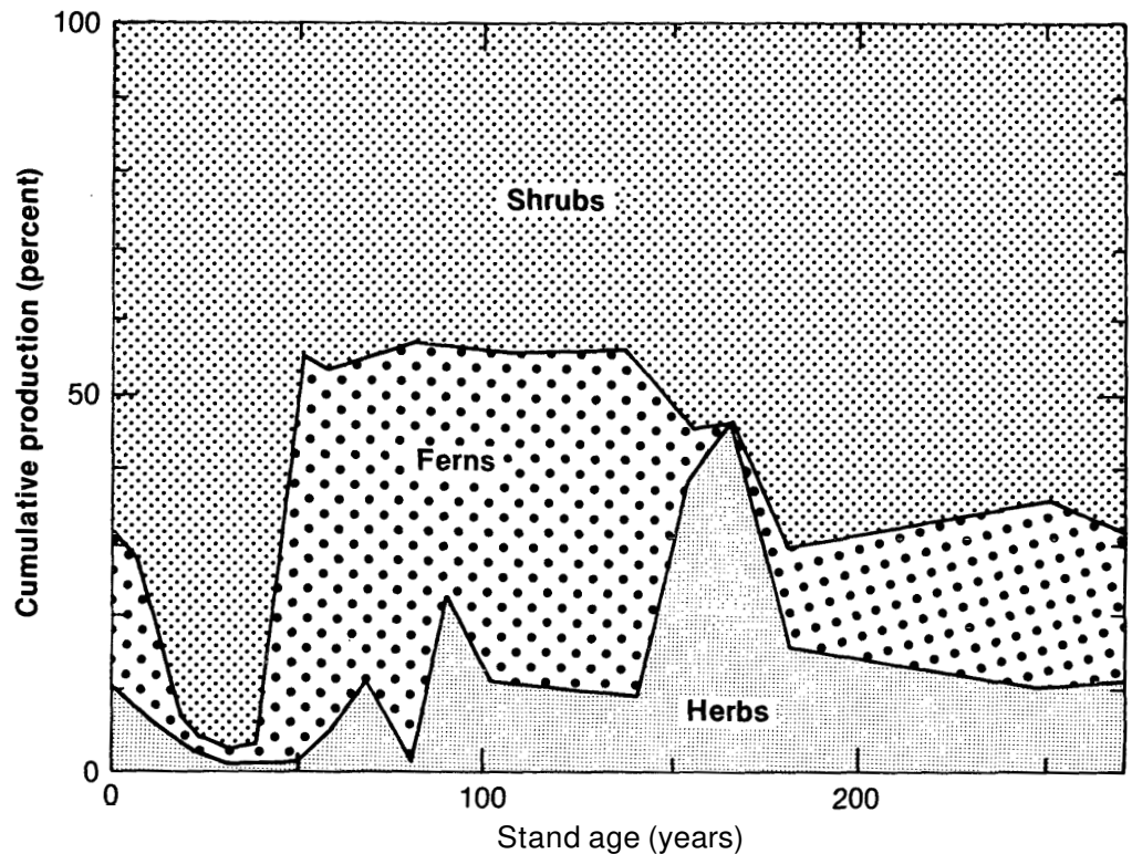
Figure 3.— Changes in under- story production during sec- ondary succession in southeast Alaska (adapted from Alaback 1982b).
