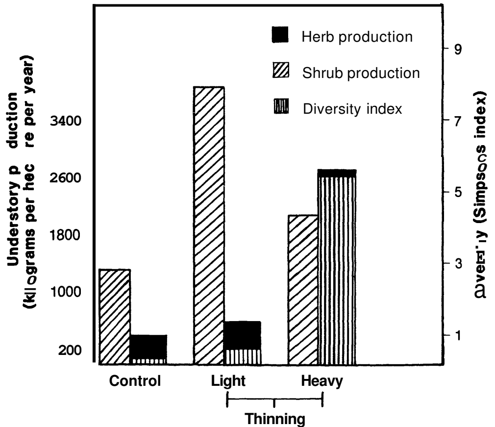
Figure 4.—Response of understory productivity to thinning in a 20-year-old stand. Diversity index is that developed by Simpson (1949).
