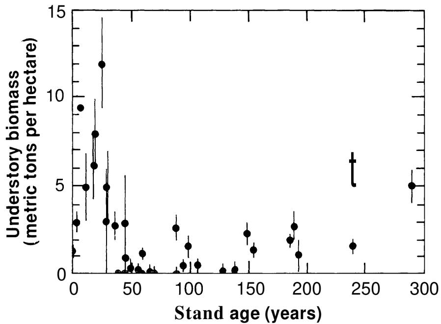
Figure 1.— Accumulation of understory biomass following disturbance in southeast Alaska. Bars represent 95-percent confidence limits on estimates of mean biomass accumulation for each site (adapted from Alaback 1982b)
